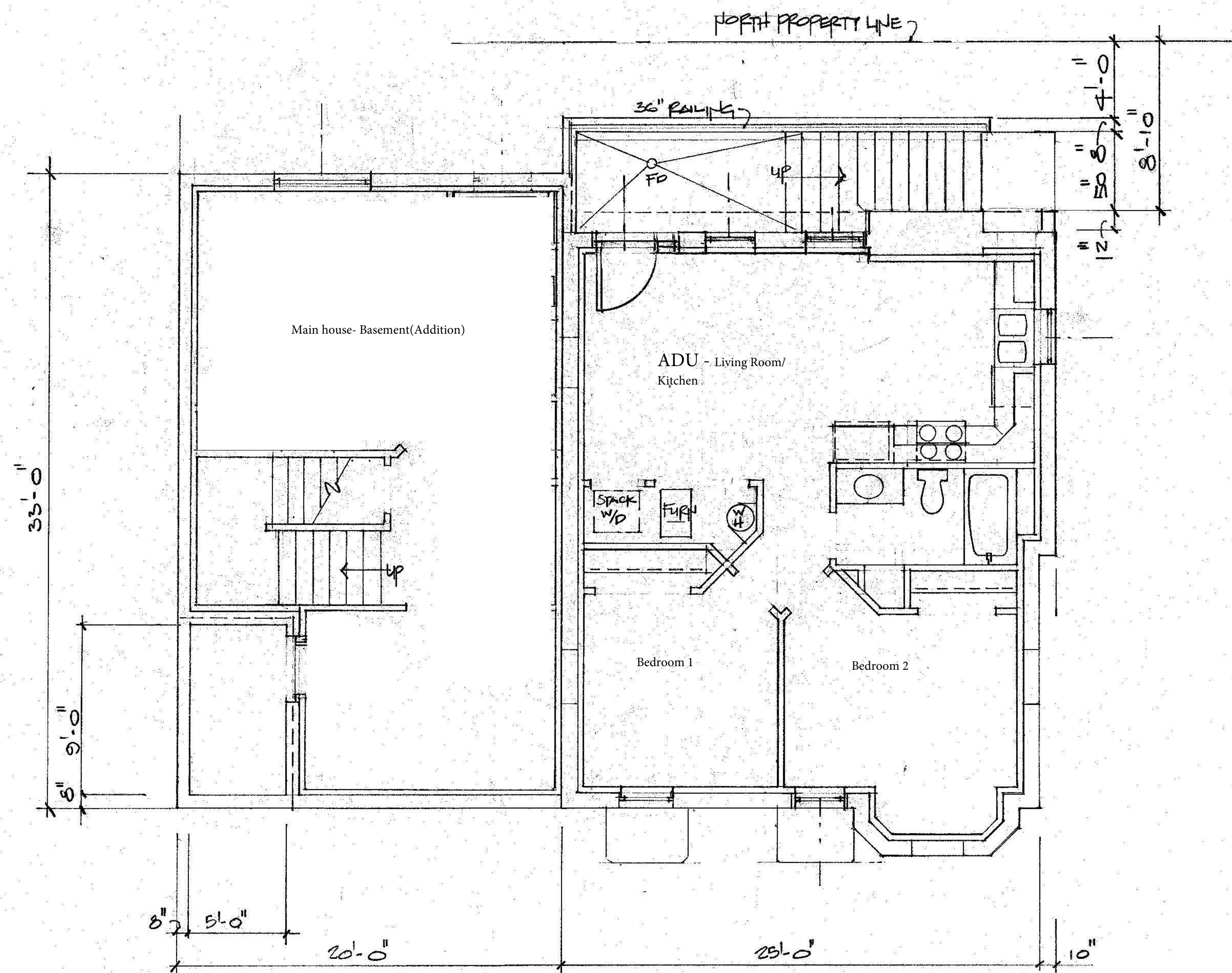
BASEMENT FLOOR PLAN 1/4"=1'-0"
